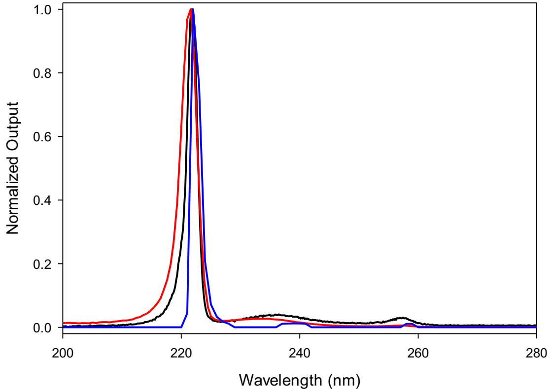
Figure 2. Emission spectra from three commercially available KrCl* lamps, data collected independently within authors' laboratories.
