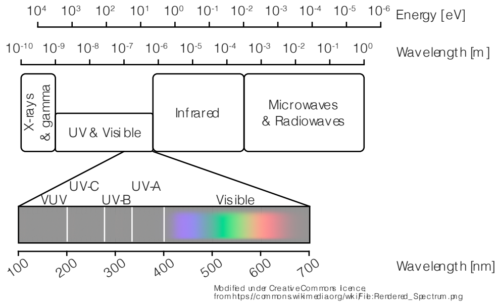
Figure 1. Electromagnetic spectrum and the position of ultraviolet radiation within it.
