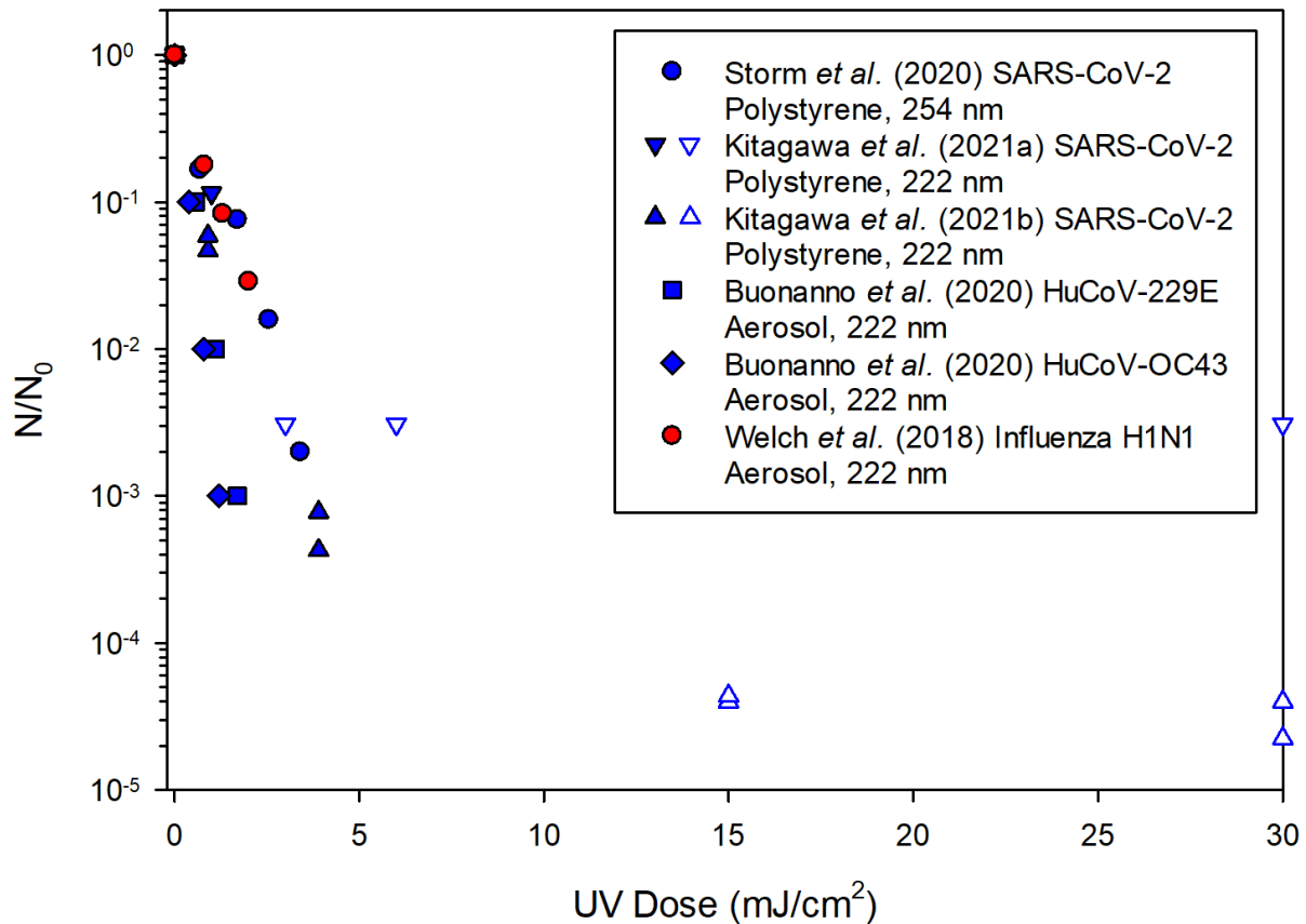
Figure 7. UV inactivation of ssRNA respiratory viruses on surfaces and in aerosols at 222 nm and 254 nm. 17, 32, 50-52 Measured inactivation responses of coronaviruses are indicated by blue symbols; measured inactivation of Influenza H1N1 virus is indicated by red symbols. The open symbols represent reported values beyond the detection limit of the viral infectivity assay.
